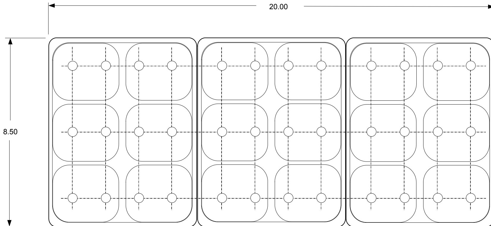
324 / 3-06 (8.5x20) Plug Positioning 12/2/03 2x4 Pattern. Leaves 3 rows in plug tray (9,18,27) Punch Plate p/n D303A0055
