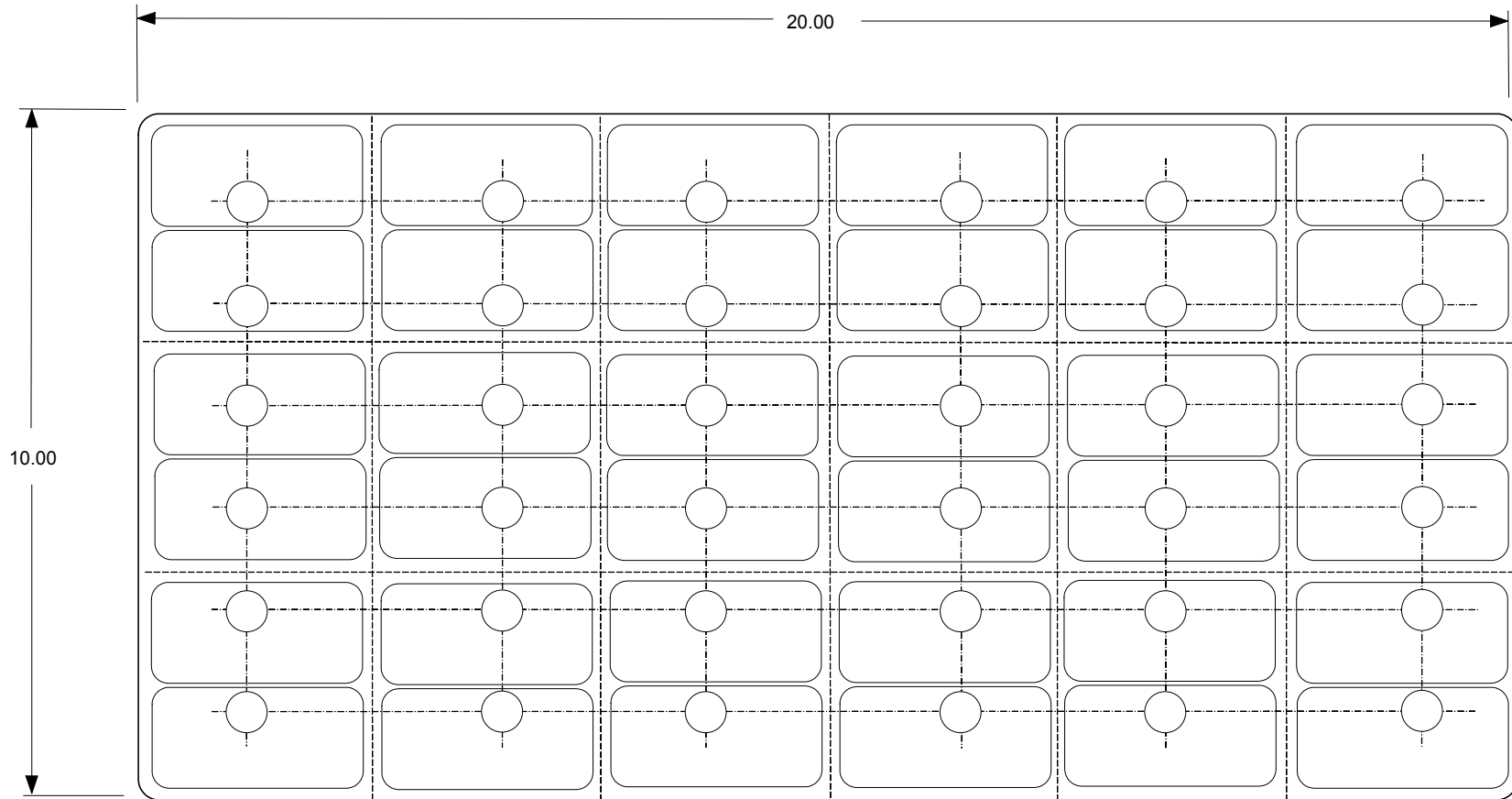
324/18-02T Ver A (10x20) Plug Positions 4x2 pattern, 3 rows remain in plug tray (5,14,23) Punch Plate p/n D303A0032
