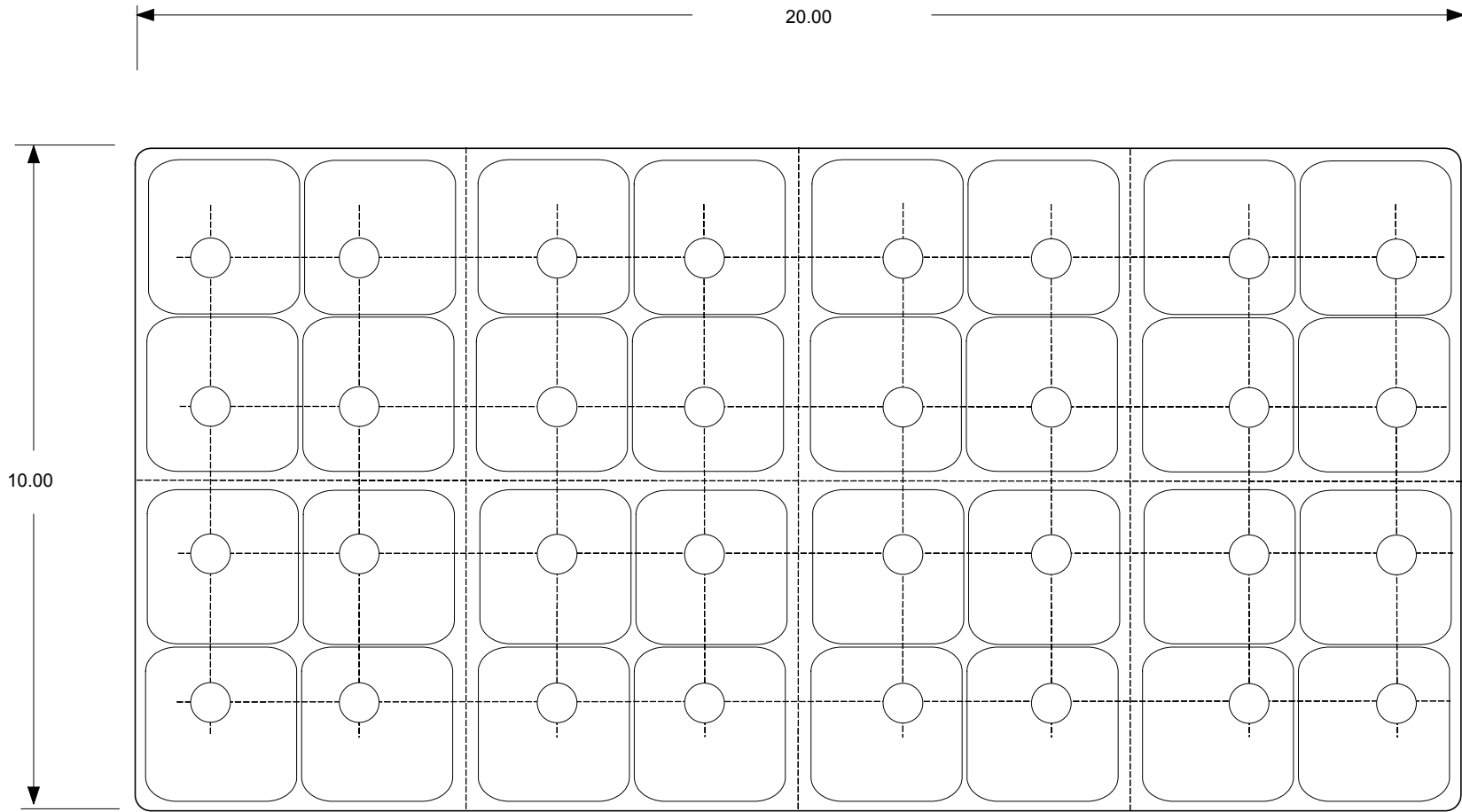
324/8-04T (10x20) Plug Positions 3x3 Pattern, 3 rows remain in plug tray (7,14,21) Punch Plate p/n D303A0039
