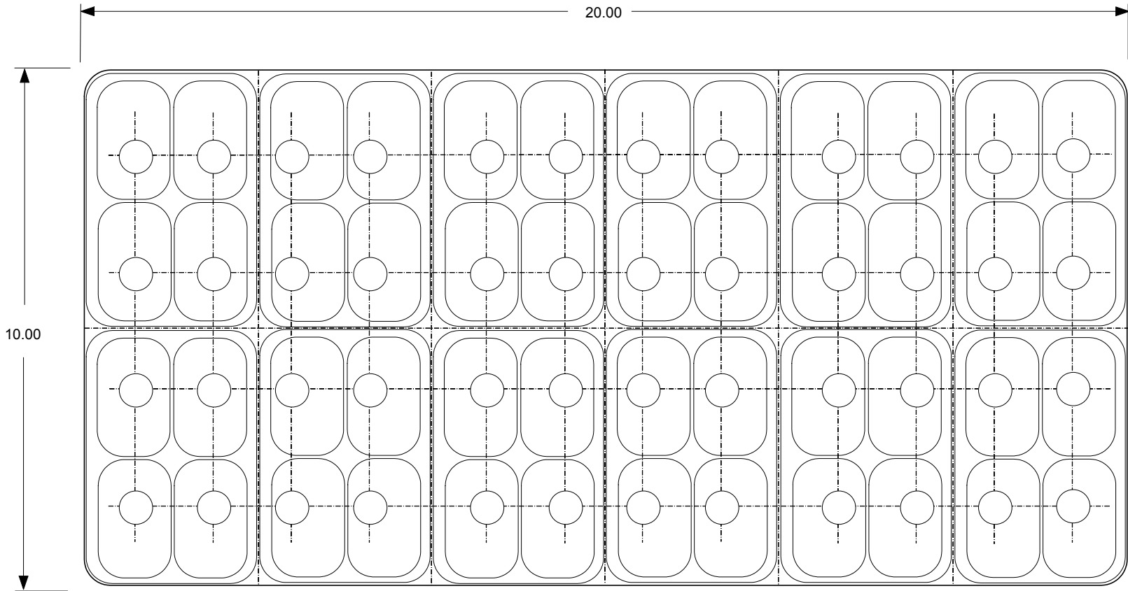
324/12-04(10x20) Plug Positions 2x3 pattern, 3 rows remain in plug tray (9, 18, 27) Punch Plate p/n D303A0045
