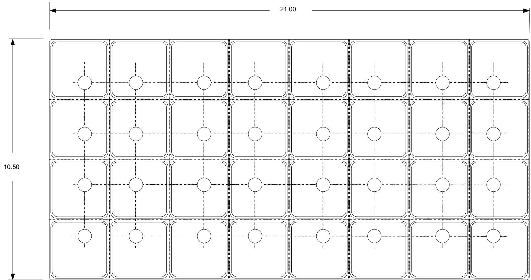
324 / 32-01 (10.5x21) Plug Positions 7/3/03 3x3 pattern, 3 rows remain in plug tray (7,14,21) P/N D303A0039
