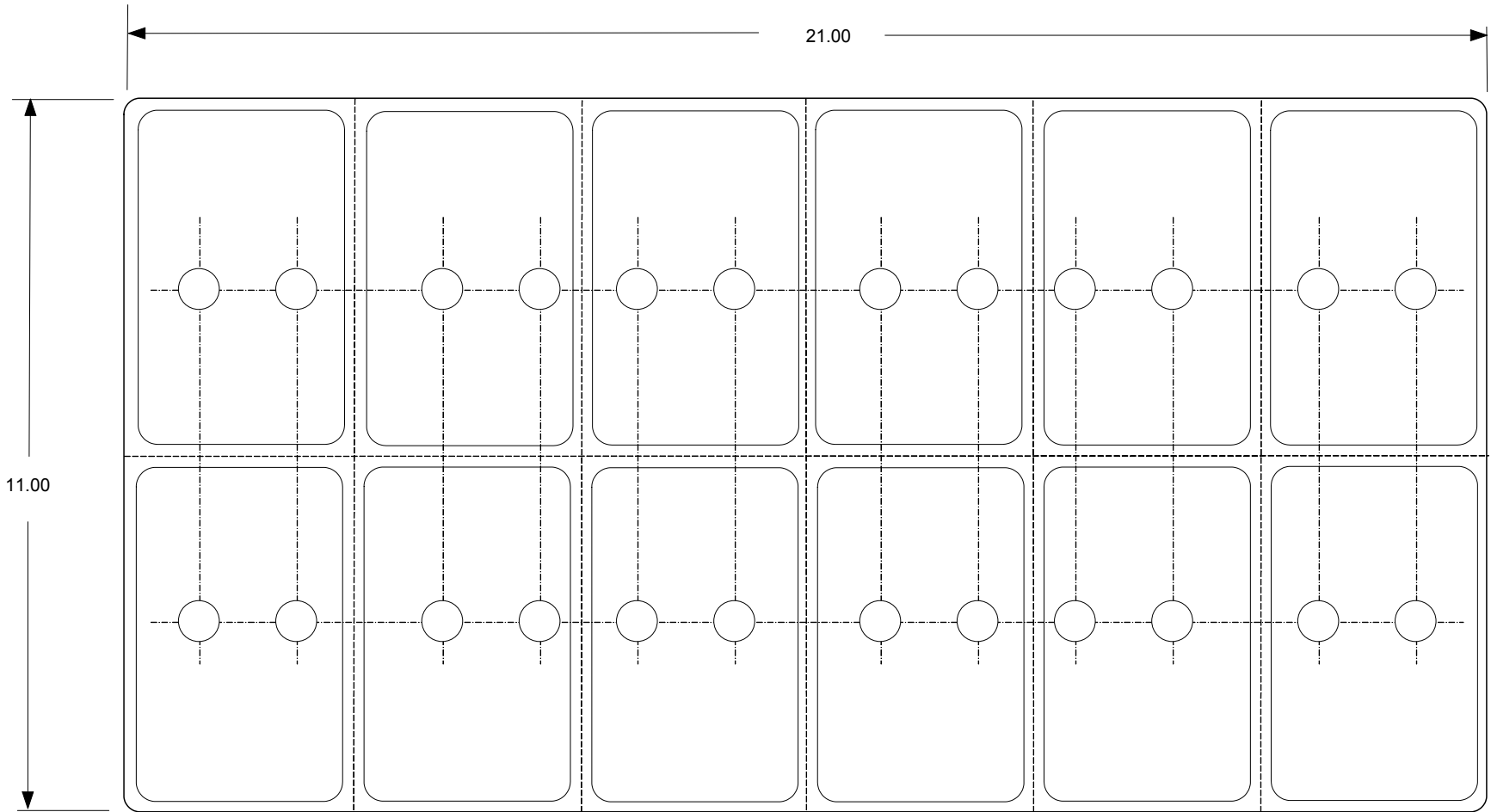
432Dp / 12-01 (11x21) Plug Positions, 2 Plugs/Cell 2x8 pattern, 3 rows remain in plug tray (5,14,23) Punch Plate p/n D303A0204
